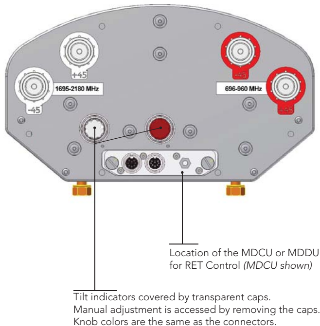
Bottom View of Antenna
