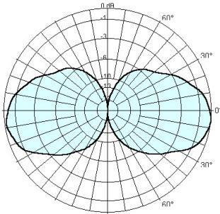
Vertical Diagramme 1800
