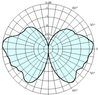
Vertical Diagramme 1800
