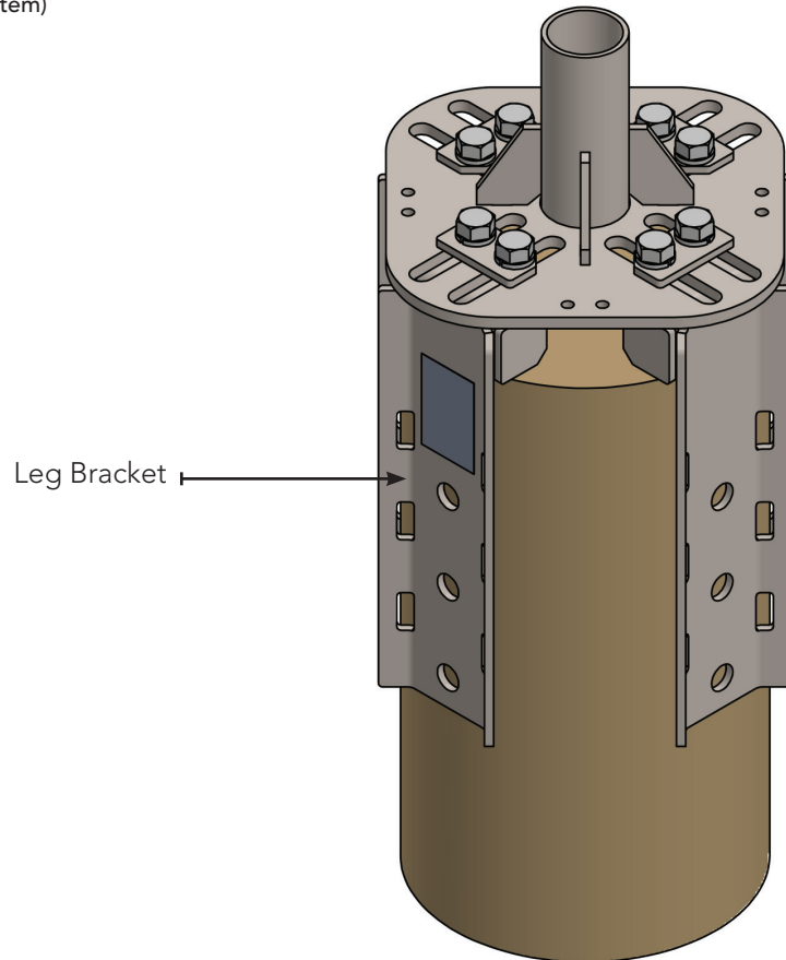
Diagram (above) shows the CWT-MKS-BASE-xx mounting kit with CWT-MKS-BASE-2BRKT option
