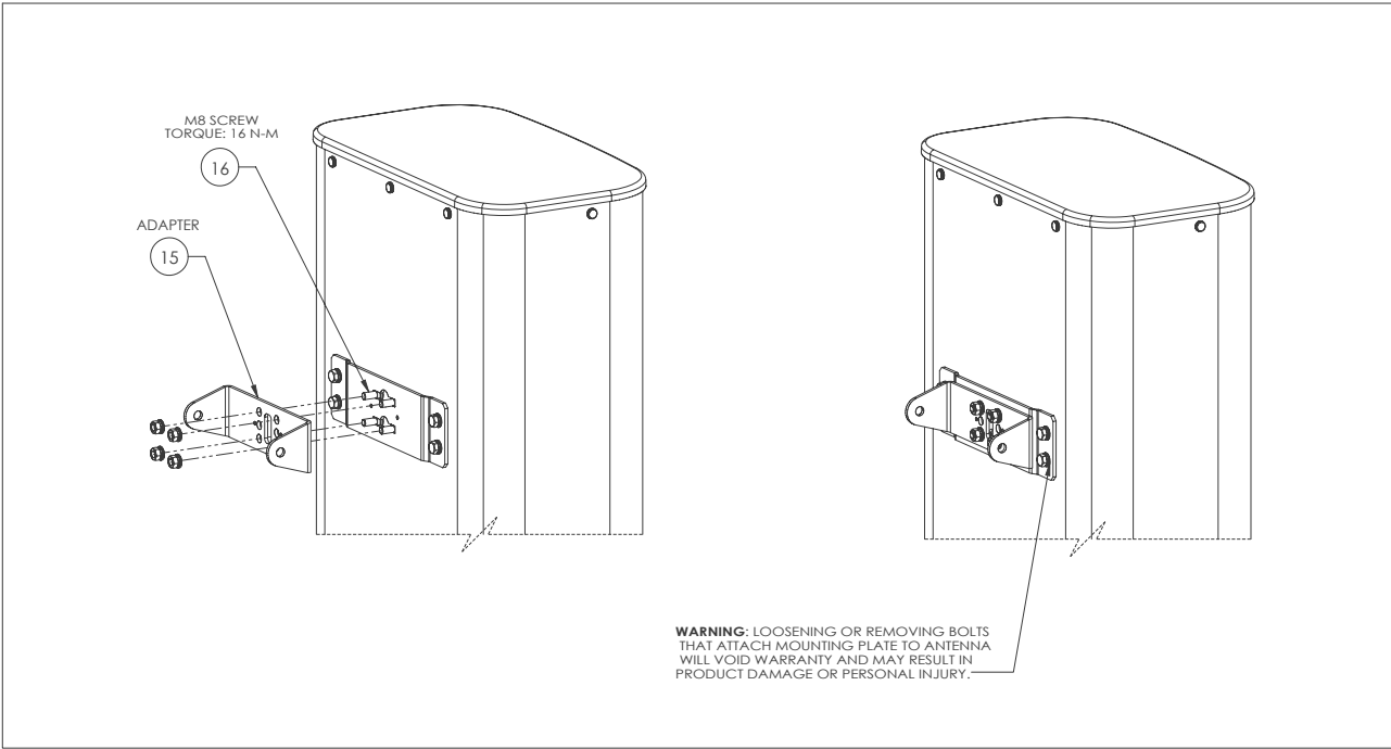
Figure 1. Pre-assembly of adapter to Antenna
