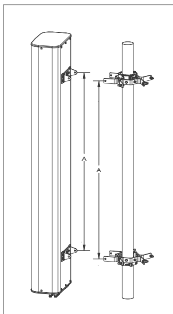
Figure 6. Obtaining Measurements for Mounting.
