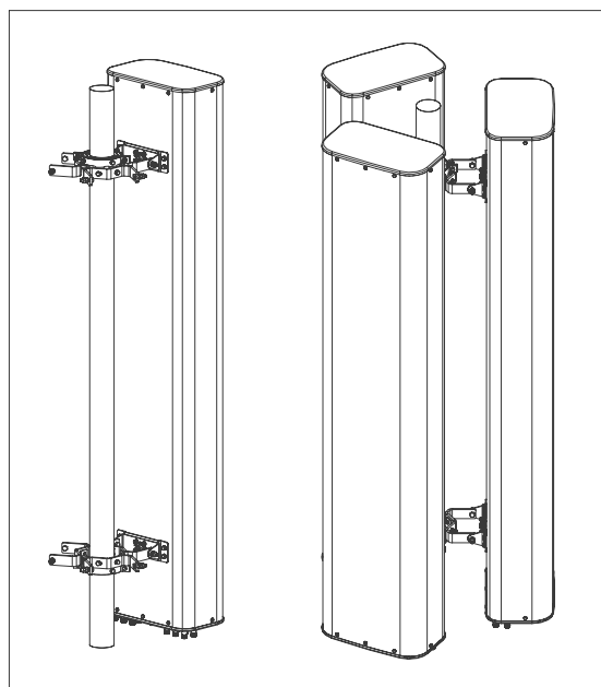
Figure 7. Attaching Antenna(s) to Pole.
