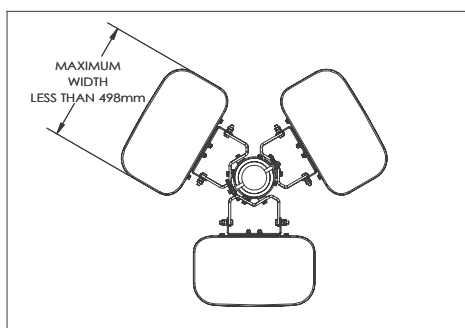
Figure 8. Maximum Antenna Width
