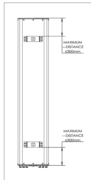
Figure 9. Maximum Distance between bracket and endcap.
