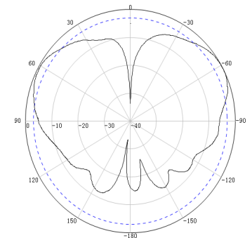
Vertical, 2500 MHz
