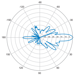
0° | Vertical | 750 MHz
