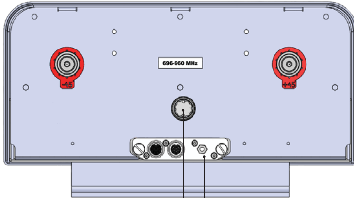
Bottom View of Antenna
