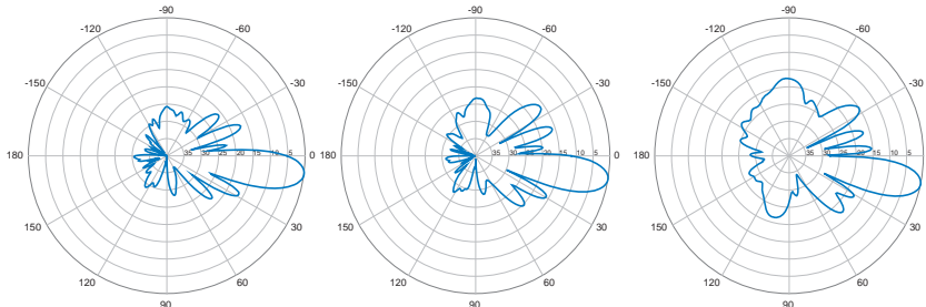
8° | Vertical | 750 MHz
