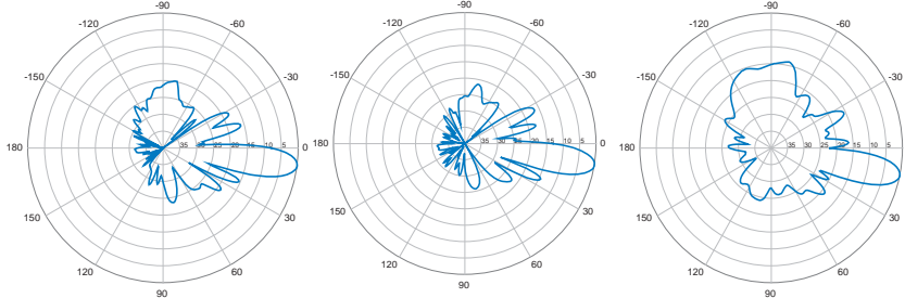
8° | Vertical | 850 MHz
