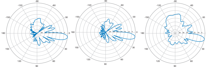
8° | Vertical | 850 MHz
