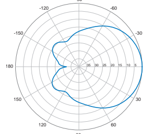
Vertical | 0° | 850 MHz
