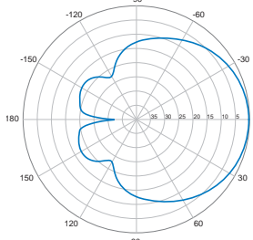
Vertical | 0° | 750 MHz
