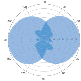
Horizontal | 1900 MHz
