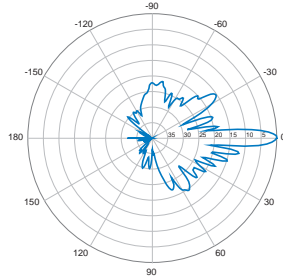
0° | Vertical | 2100 MHz
