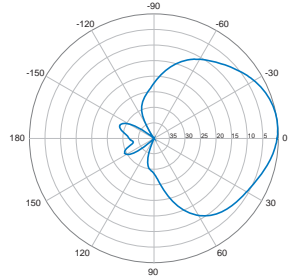
Horizontal | 2600 MHz
