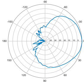
Horizontal | 1900 MHz
