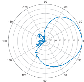
Horizontal | 2100 MHz
