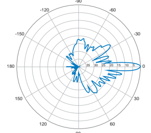
0° | Vertical | 2100 MHz
