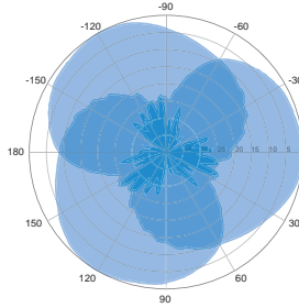
Horizontal | 1900 MHz
