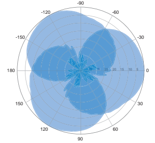
Horizontal | 2100 MHz
