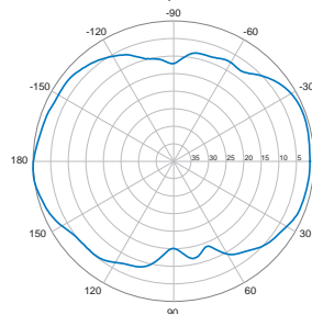
0° | Vertical | 750 MHz
