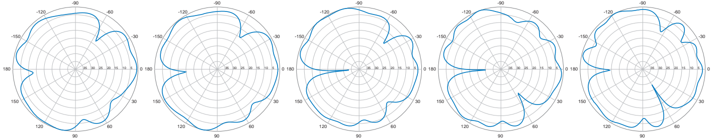
Horizontal | 180 MHz
