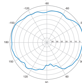
0° | Vertical | 850 MHz
