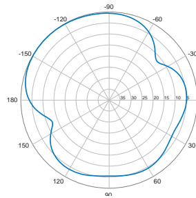
Horizontal | 750 MHz
