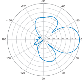
Vertical | 0° | 1800 MHz
