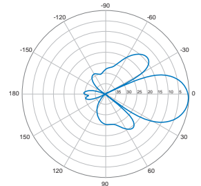
Vertical | 5° | 2100 MHz
