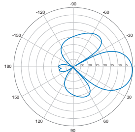
Vertical | 5° | 1900 MHz
