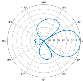
Vertical | 5° | 1800 MHz
