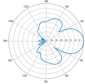
Vertical | 0° | 1900 MHz
