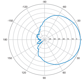
Horizontal | 850 MHz
