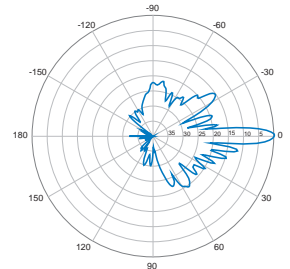
0° | Vertical | 2100 MHz
