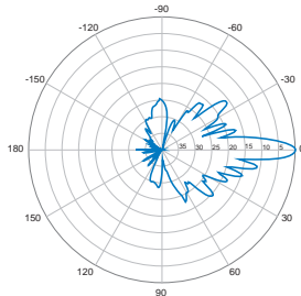
0° | Vertical | 1900 MHz
