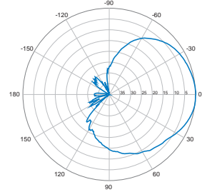
Horizontal | 2100 MHz
