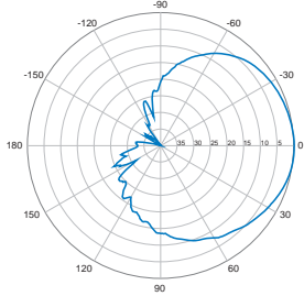
Horizontal | 1800 MHz
