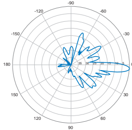
6° | Vertical | 1900 MHz
