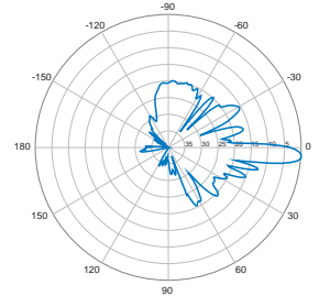
6° | Vertical | 2100 MHz
