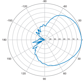
Horizontal | 1900 MHz
