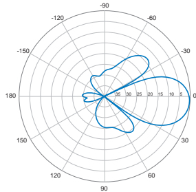
Vertical | 5° | 2100 MHz
