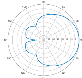
Vertical | 0° | 750 MHz
