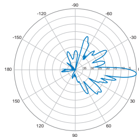
6° | Vertical | 1900 MHz
