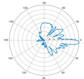
6° | Vertical | 2100 MHz
