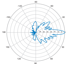
0° | Vertical | 1900 MHz
