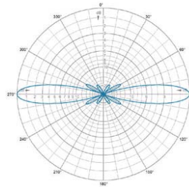
0° | Vertical | 875 MHz
